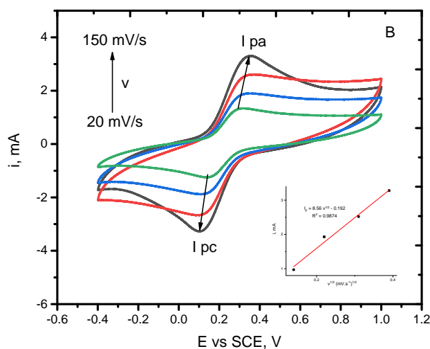
Cyclic Voltammograms recorded in 5 mmol.L -1 K 3 [Fe(CN) 6 ]/K 4 [Fe(CN) 6 ] system at different scan rates on thin film r GO 600 °C.
