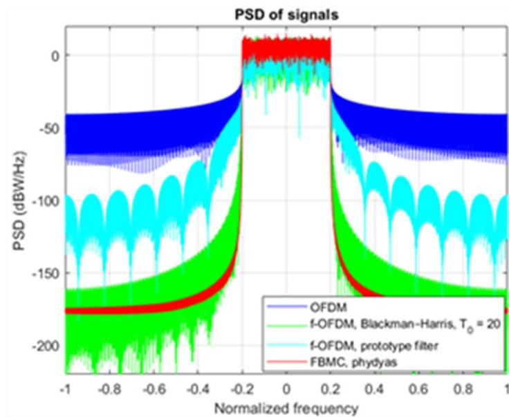
Compare the power signal density (PSD) of f-OFDM with OFDM and FBMC.
